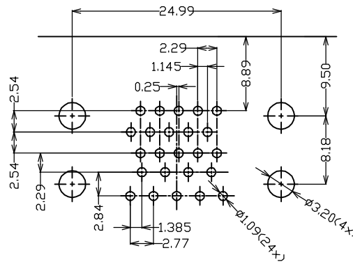
RECOMMEND P.C.B. LAYOUT BOTTOM VIEW
