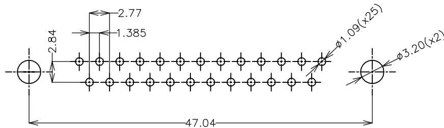
P.C.B. LAYOUT(TORANCE±0.05) TOP VIEW
