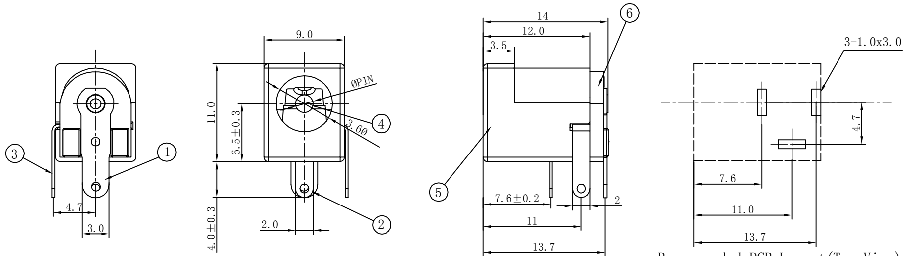
Recommended PCB Layout (Top View) General tolerance: ±0.05
